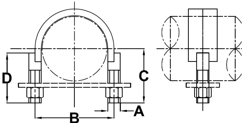
DIMENSIONAL CHART
