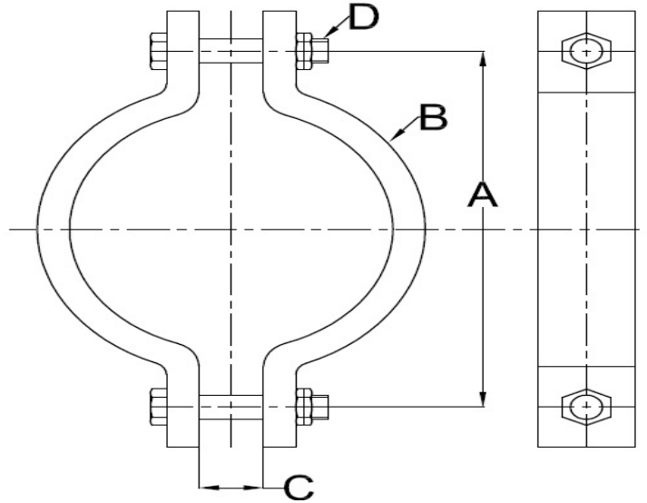
DIMENSIONAL CHART
